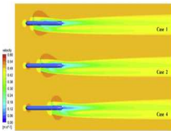
Fig. 15. Contours of velocity at the lateral cross-section planes at TSR \frac{1}{4} 5 .
