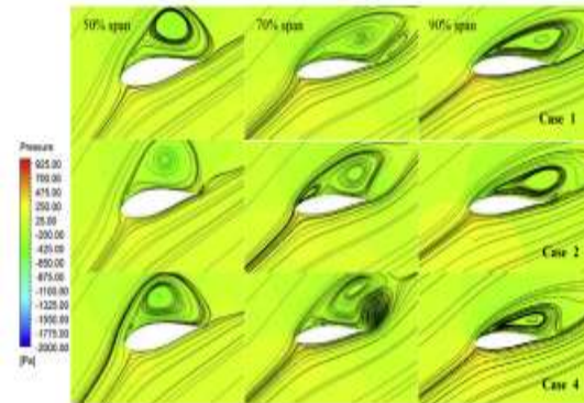
Pressure contours and streamlines along the chosen portions at TSR 14 2 are shown in Fig. 12.
