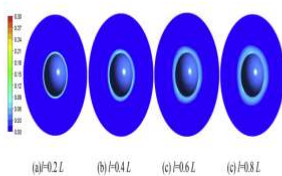
Figure 8: Cross-sectional intensity contours of turbulence at TSR = 5 for l = 0.2L , 0.4L , 0.6L , and 0.8L upstream of the turbines.
