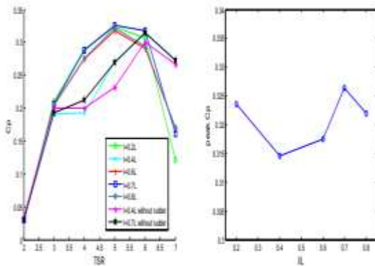
Fig. 7. The results of C_p : (a) C_p vs. TSR and (b) peak C_p vs. l .
