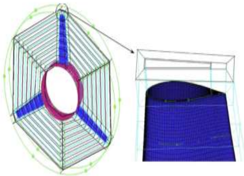
Fig. 4. Grid of the rotor sub domain.
