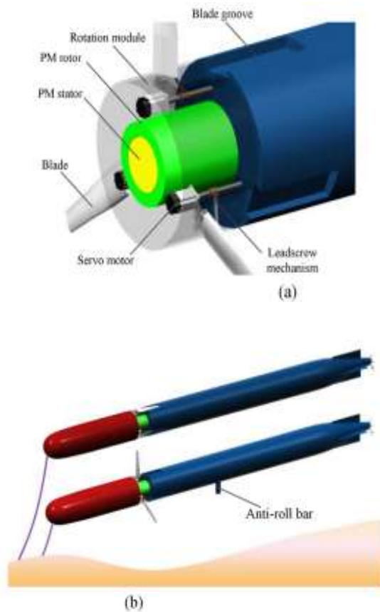
Fig. 1 (a) shows the HAWT's internal construction, and (b) depicts the turbine as it might appear on a UMP.
