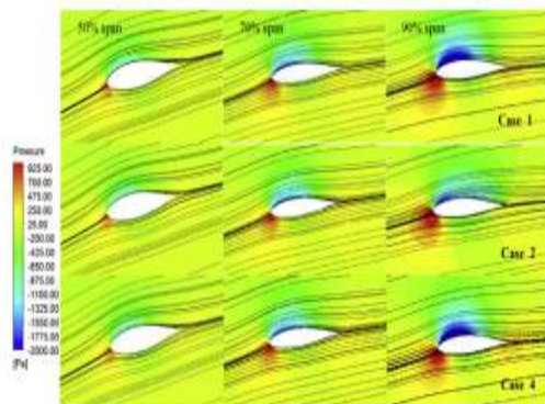
Fig. 13. Streamlines and contours of pressure on the selected sections at TSR \frac{1}{5} .
