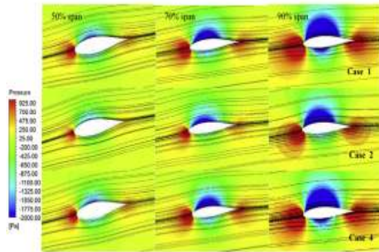
Fig. 14. Streamlines and contours of pressure on the selected sections at TSR \frac{1}{4} 7 .
